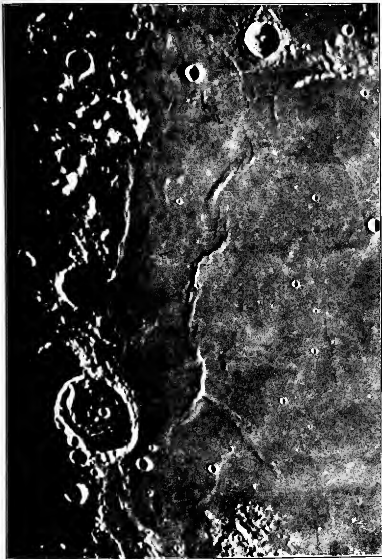
WESTERN PART OF THE MARE SERENITATIS
